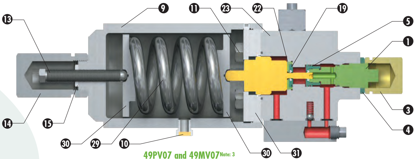
Modulator Assembly For 49MV07
