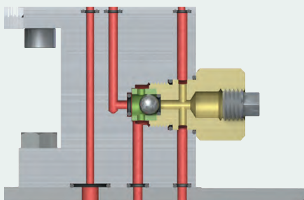
Backflow Preventer
