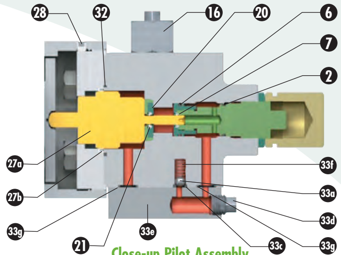
Close-up Pilot Assembly 49PV07 and 49MV07 Note: 3
