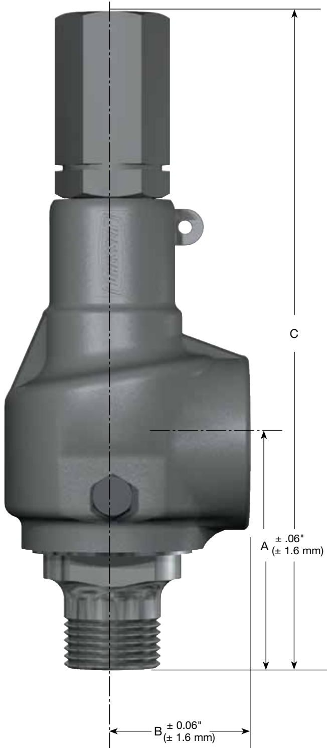
Main Valve Dimensions
